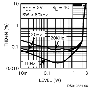
LM4863MTE THD+N vs Output Power
