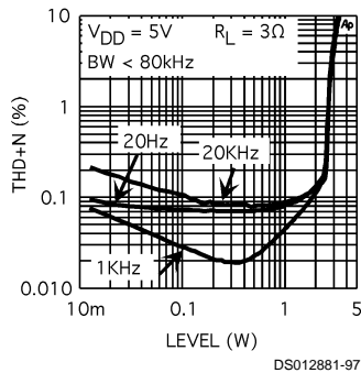
LM4863MTE THD+N vs Output Power
