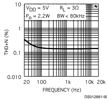
LM4863MTE THD+N vs Frequency
