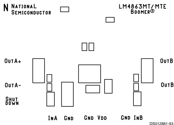
Figure 4. MTE PC board layout: Component-side Silkscreen
