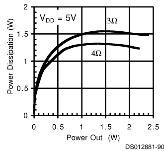
LM4863MTE Power Dissipation vs Power Output
