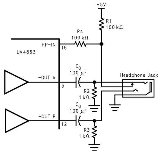
FIGURE 2. Headphone Circuit
