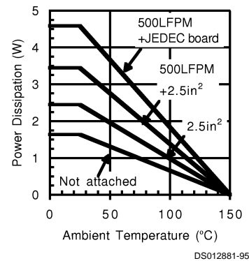
LM4863MTE (Note 20) Power Derating Curve
