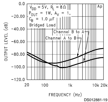
Channel Separation
