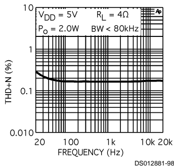
LM4863MTE THD+N vs Frequency
