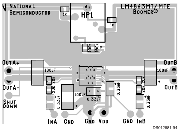
Figure 3. MTE PC board layout: all layers superimposed
